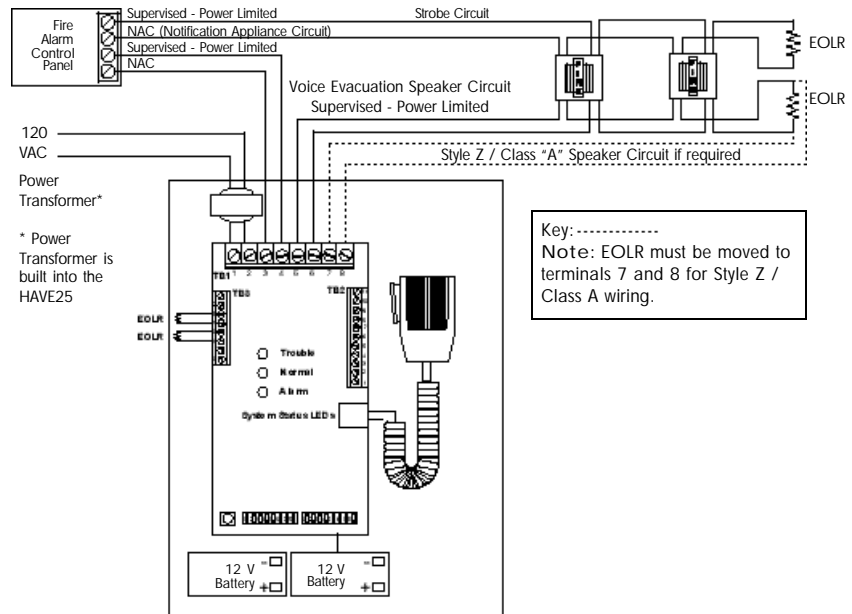
Wiring Diagram HAVE50 Series
